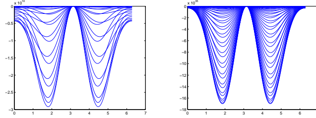
FIGURE 3. The functions \beta_0(\theta, \rho_n), \dots, \beta_{29}(\theta, \rho_n) in the case n = 4 (left) and the functions \beta_0(\theta, \rho_n), \dots, \beta_{121}(\theta, \rho_n) in the case n = 27 (right)
